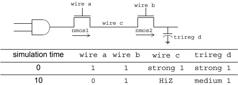
Figure 4-1—Simulation values of a trireg and its driver
